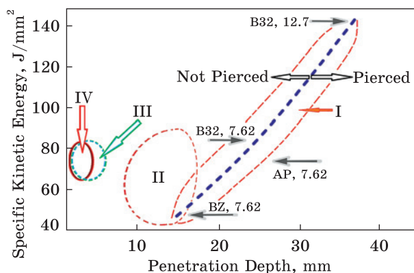
Fig. 13. Specific kinetic energy of bullets and results of ballistic tests (piercing-not piercing) depending on the thickness of titanium-based materials. All data for BZ and B32 ammunitions are adopted from [15, 17, 34]. Dashed line is plotted for the data from [28]
