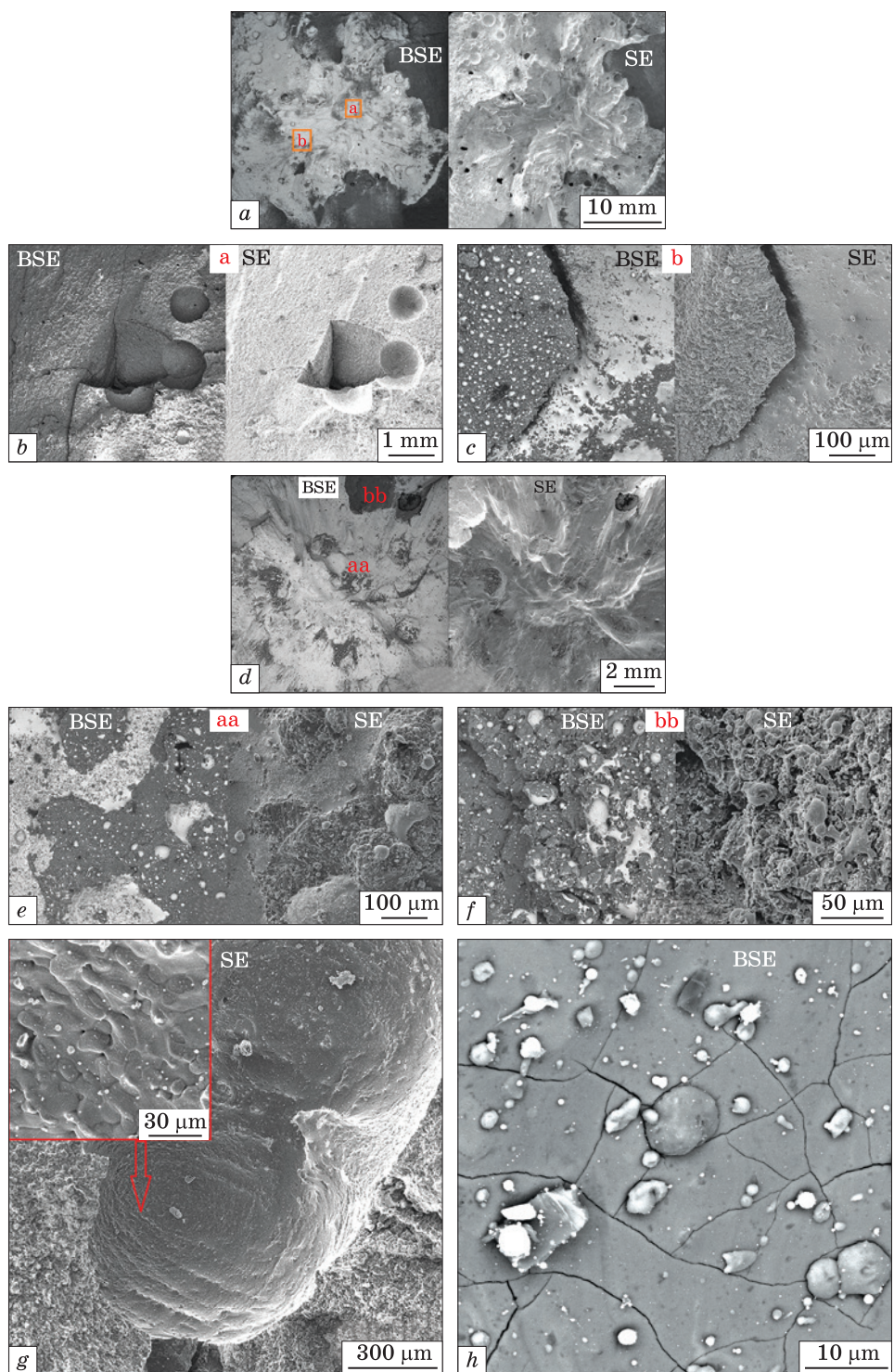
Fig. 5. SEM images of craters formed by bullets' impact in the samples (a–c) #2, and (d–h) #3; b and c — relevant images shown in a; e and f — in d; g — typical pore; h — high resolution image of 'flat' cleavage zone at the distance of 2 cm from bullet hit point
