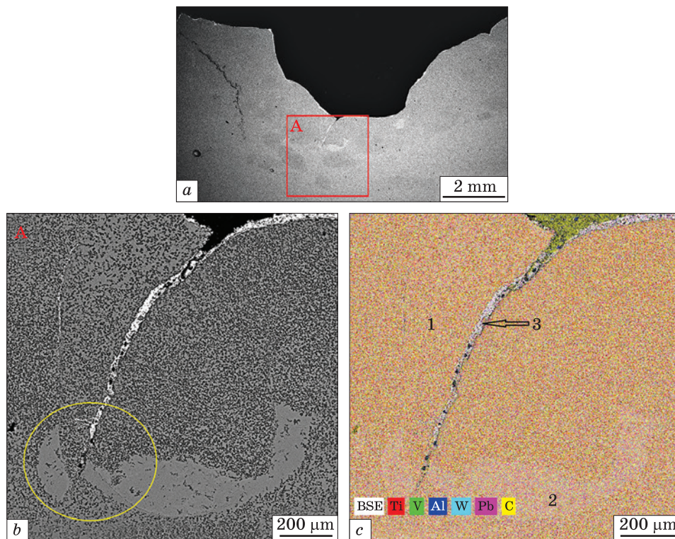
Fig. 6. Cross-section of the ballistic tested sample showing general view of the crater (a), analysed region (A) around the crack (b), and distribution of chemical elements (EDS analysis) in this zone (c). Areas in (c): 1 — uniformly distributed all alloying elements and fine TiC particles, 2 — zone depleted of TiC particles and enriched by Ti and Al, 3 — crack filled with molten lead. SEM, BSE
