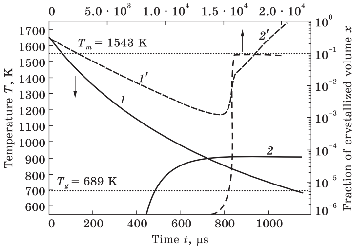
Fig. 2. Calculated time ( t ) dependences of temperature T ( 1, 1' ) and fraction of the crystallized volume x ( 2, 2' ) for \text{Fe}_{80}\text{B}_{20} alloy layers of 20\ \mu\text{m} ( 1, 2 ) and 100\ \mu\text{m} ( 1', 2' ) thick [7]
