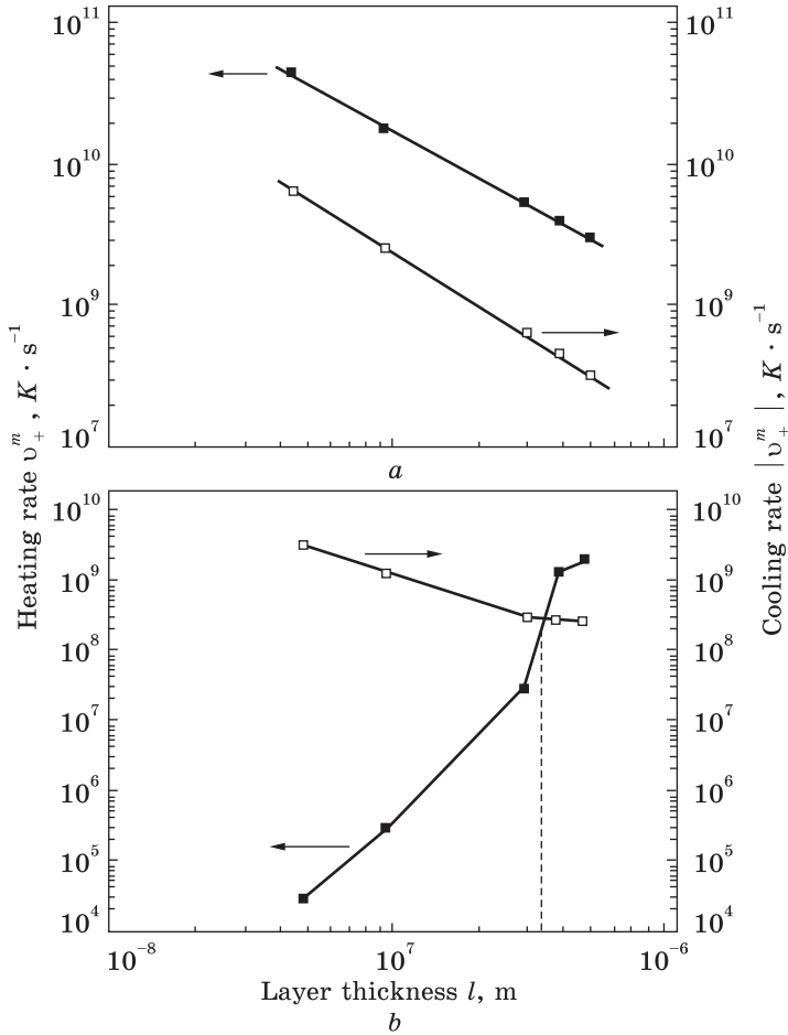
Fig. 5. Calculated dependences of the v_+^m and |v_-^m| parameters on the layer thickness of Al (a) and Ni (b) melts [66]
