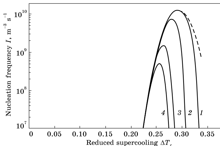
Fig. 7. Dependences of the I_0\Delta(T_r) (dashed line) and I\Delta(T_r) (solid lines) for the Zr_{41.2}Ti_{13.8}Cu_{12.5}Ni_{10}Be_{22.5} alloy layers quenched from the liquid state with cooling rates v \geq v_c : 1.3 K/s (1), 64.4 K/s (2), 9.8 \cdot 10^{-2} K/s (3), and 2.7 \cdot 10^3 K/s (4) [7]
